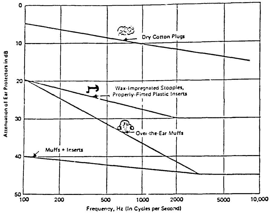
FIG. 2-10. SOUND ATTENUATION CHARACTERISTICS OF VARIOUS TYPES OF EAR PROTECTORS Source: Ref. 23
