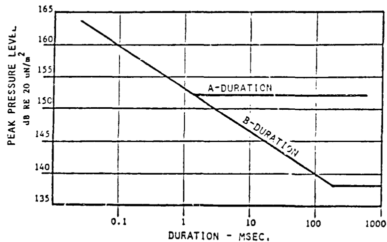
FIG. 2-6. BASIC LIMITS FOR IMPULSE NOISE EXPOSURE ASSUMING 100 IMPULSES PER DAY AND OTHER CONDITIONS AS STATED IN THE TEXT.
