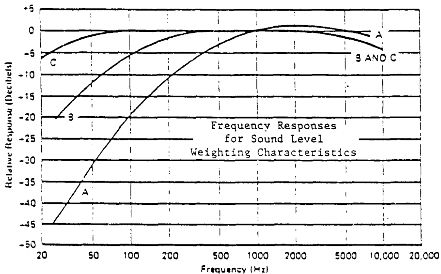
FIG. 7-1. FREQUENCY RESPONSES FOR SOUND LEVEL WEIGHTING CHARACTERISTICS.
