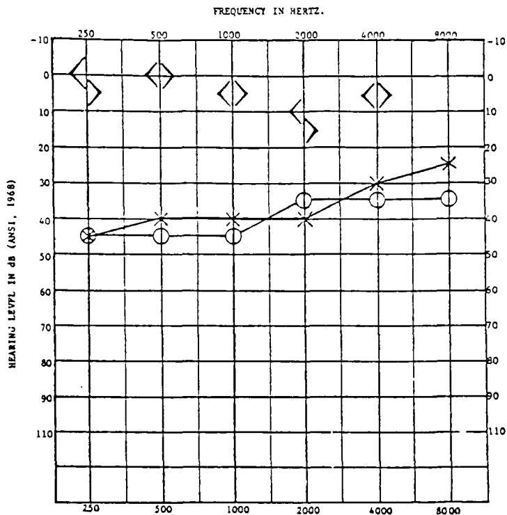
FIG. 2-3. SAMPLE AUDIOGRAM
